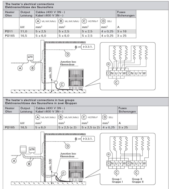
Electrical connections
